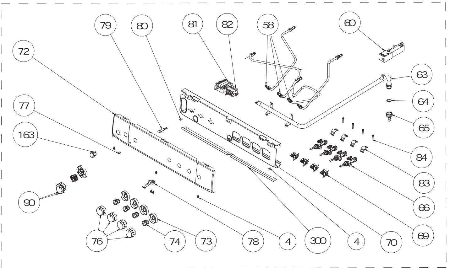
3D- 4GAS - NO TIMER CONTROL PANEL ASSEMBLY
