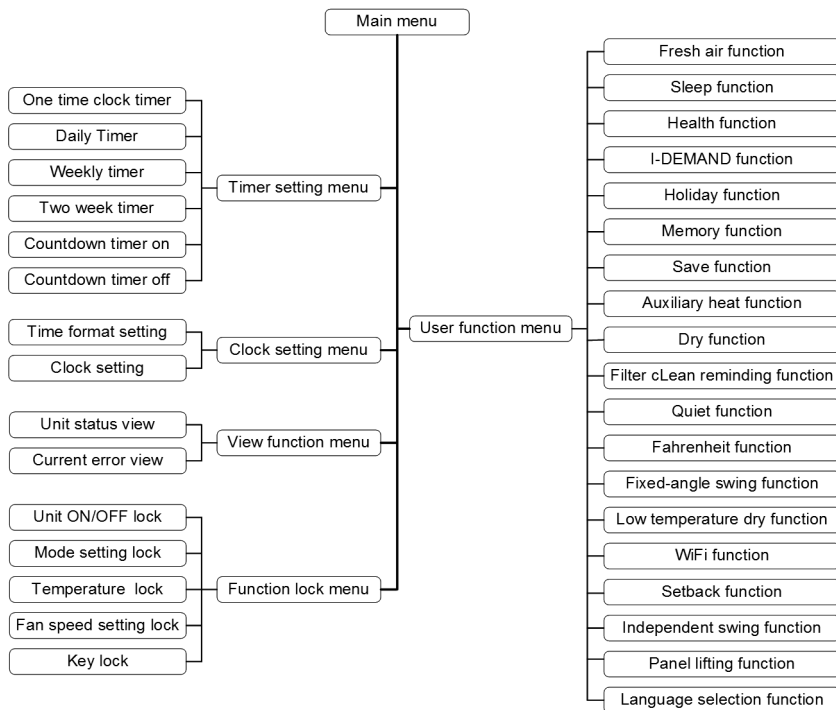
Figure 4-1 Menu structure
