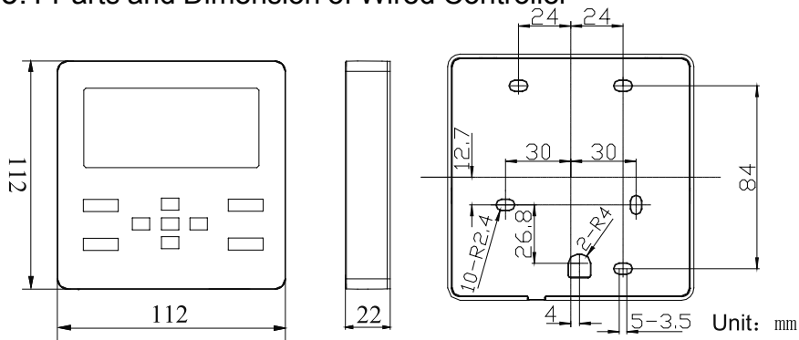
Figure 5-1 Dimension of wired controller
