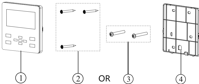
Figure 5-2 Parts of wired controller
